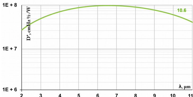
Example of D^* vs Wavelength \lambda for PEMI Series HgCdTe Detectors. Spectral Characteristics of individual detectors may vary from those shown on the chart.
