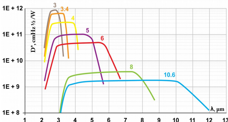
Example of D^* vs Wavelength \lambda for PVI-2TE Series HgCdTe Detectors. Spectral Characteristics of individual detectors may vary from those shown on the chart.
